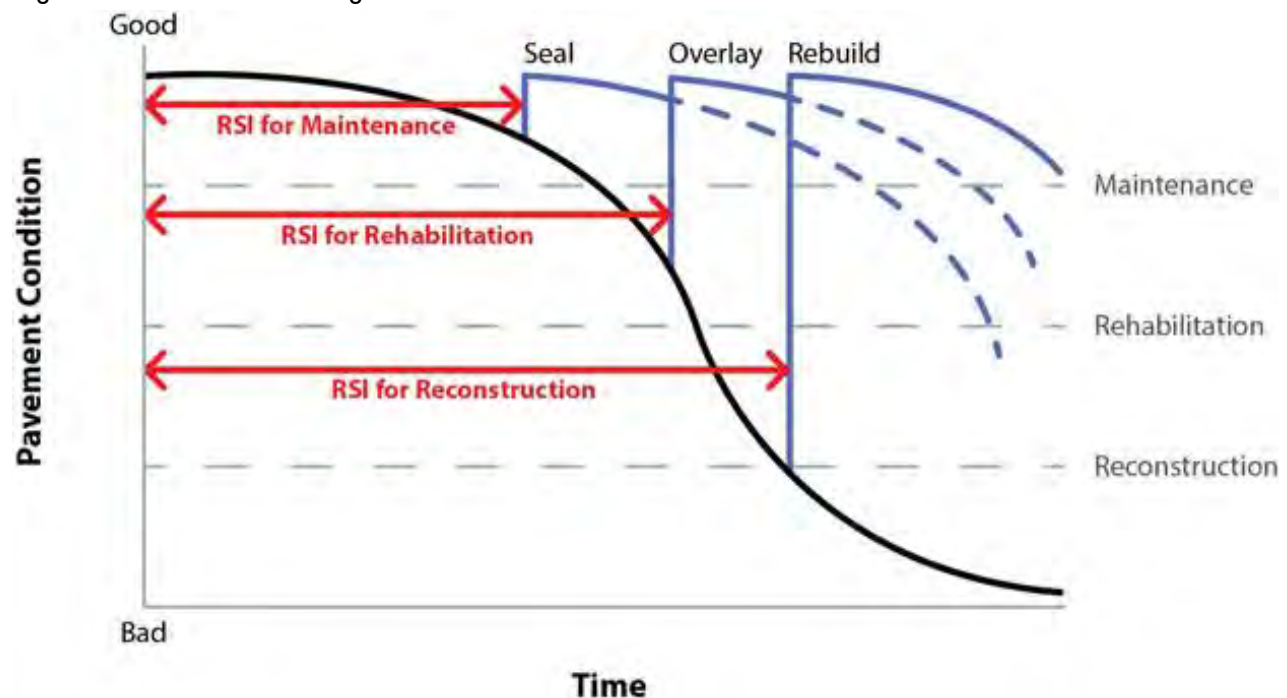
Figure 5-2 - Life-extending Benefit of Preventive Maintenance Treatment
