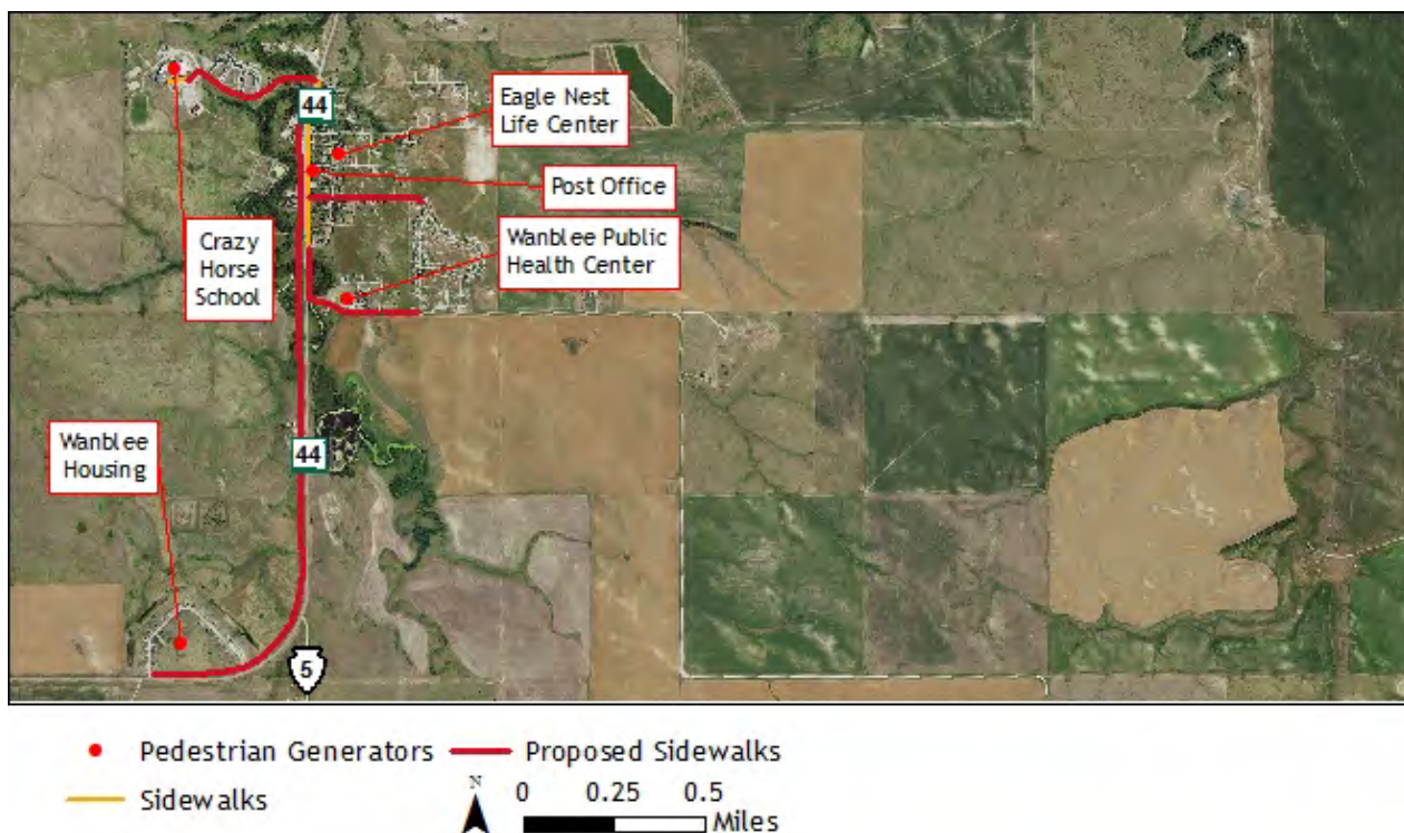
FIGURE 3-21 – Existing and Proposed Sidewalks – Wanblee
