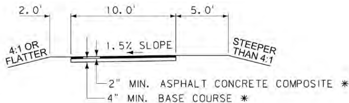
FIGURE 9-6 - Standard Separated Shared Use Path Typical Section
