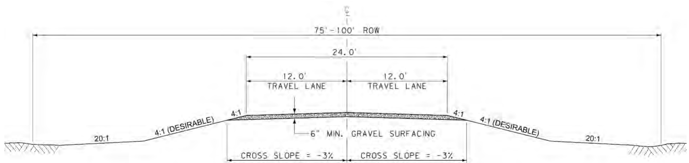
FIGURE 9-3 -Low Speed Gravel Road Typical Section
