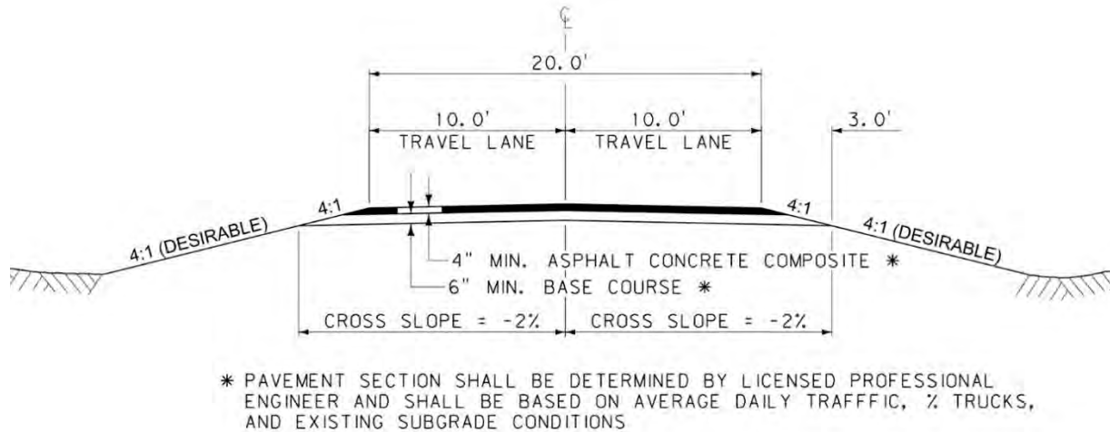
FIGURE 9-5 -Tribal Housing & Residential Street Typical Section - Urban
