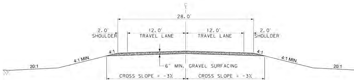
FIGURE 9-3 -Low Speed Gravel Road Typical Section
