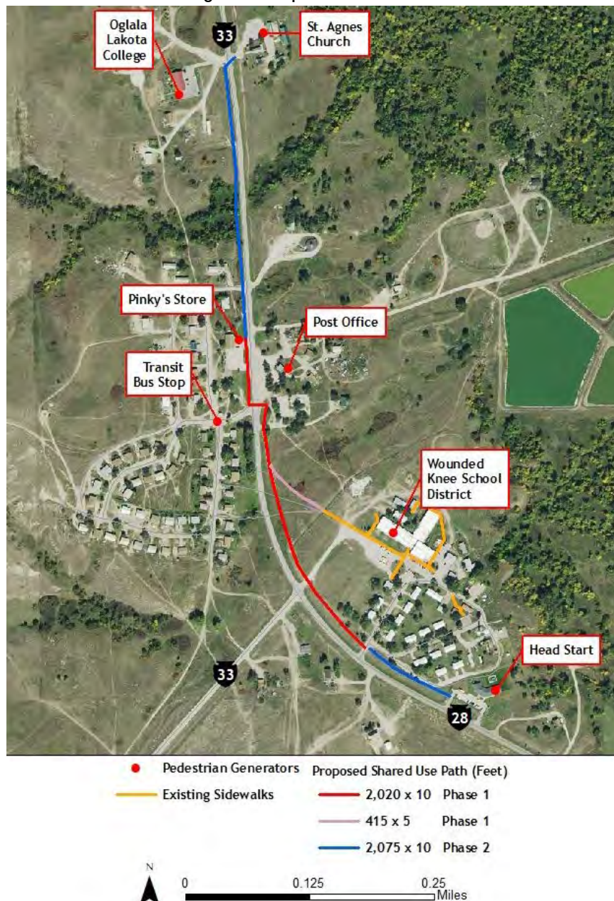
FIGURE 3-16 – Existing and Proposed Sidewalks – Manderson
