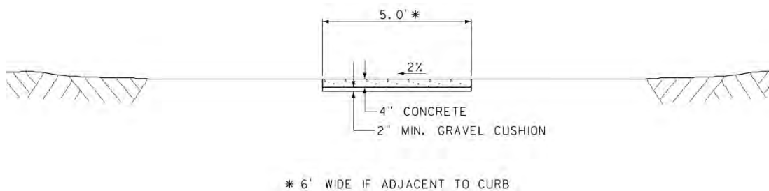
FIGURE 9-7 – Standard Sidewalk Typical Section
